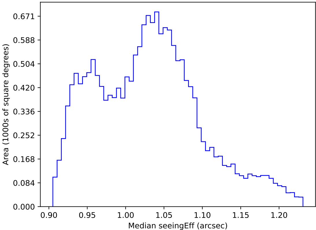
weather_cloudso4v3.4_10yrs WFD all bands: Median seeingEff
