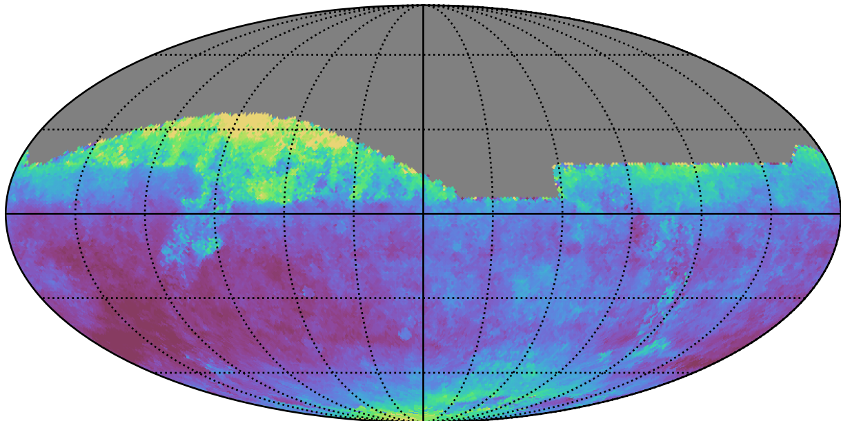
weather_cloudso4v3.4_10yrs All sky z band: Median seeingEff
