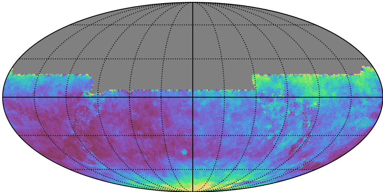
weather_cloudso4v3.4_10yrs All sky y band: Median seeingEff
