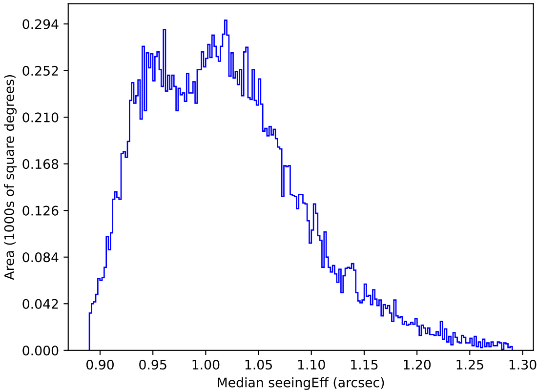
weather_cloudso4v3.4_10yrs All sky y band: Median seeingEff
