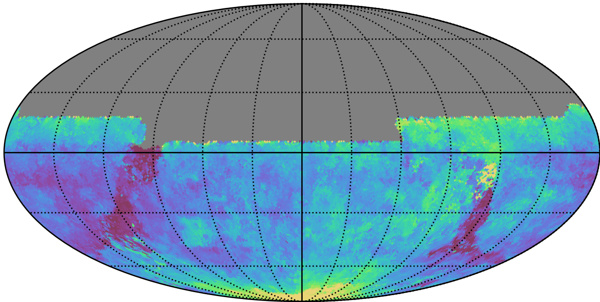
weather_cloudso4v3.4_10yrs All sky u band: Median seeingEff
