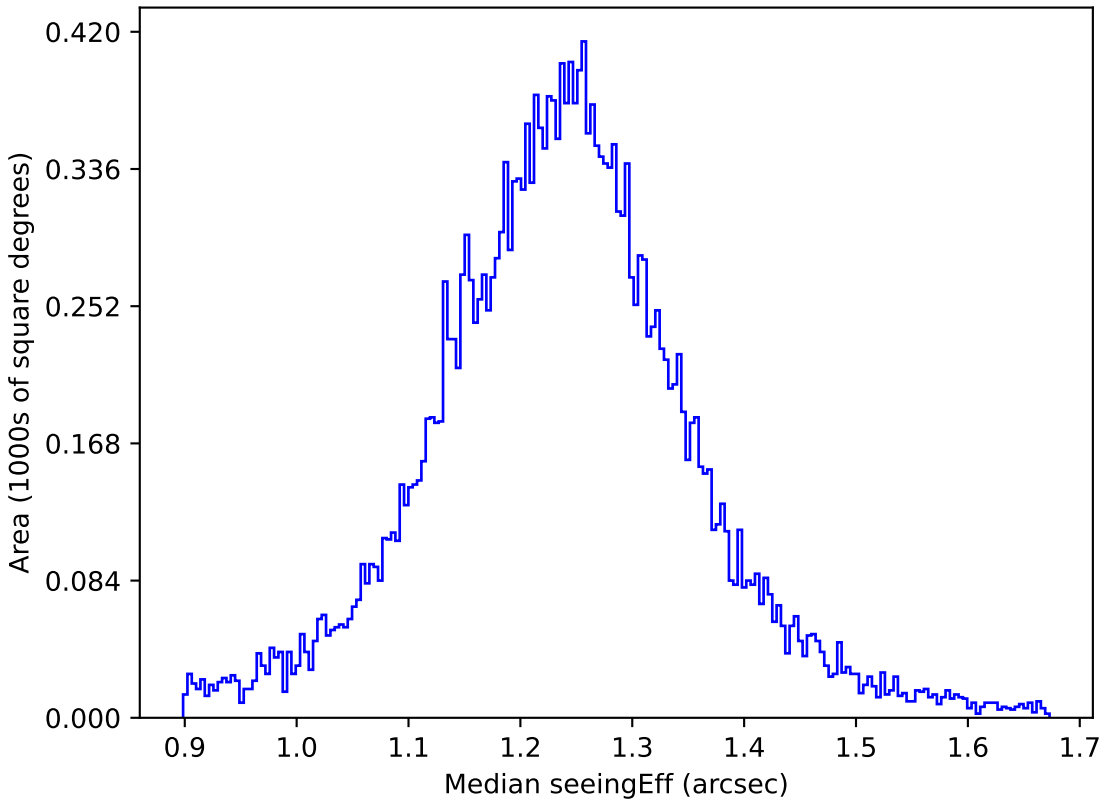
weather_cloudso4v3.4_10yrs All sky u band: Median seeingEff
