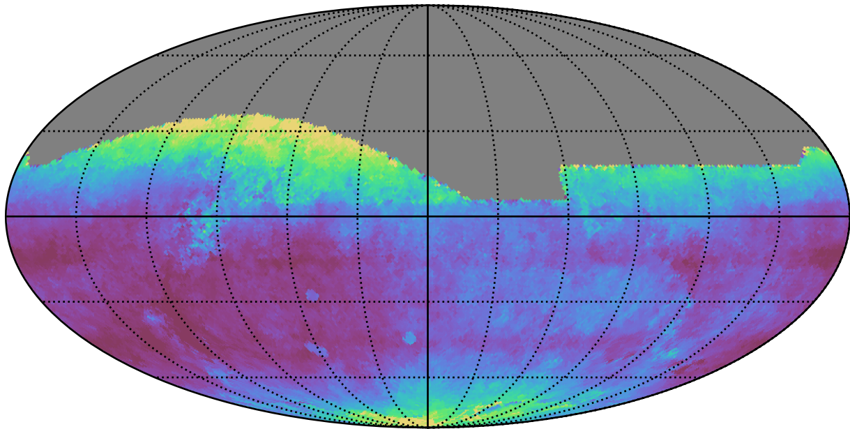
weather_cloudso4v3.4_10yrs All sky r band: Median seeingEff
