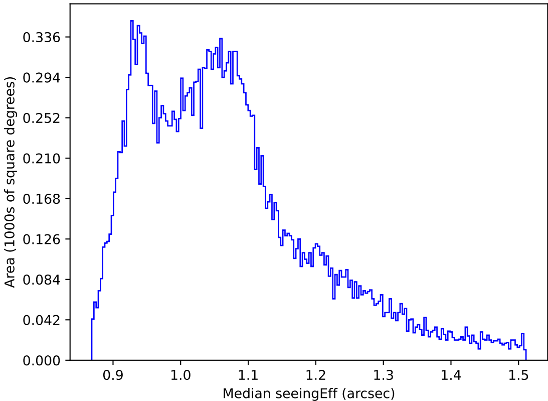
weather_cloudso4v3.4_10yrs All sky r band: Median seeingEff
