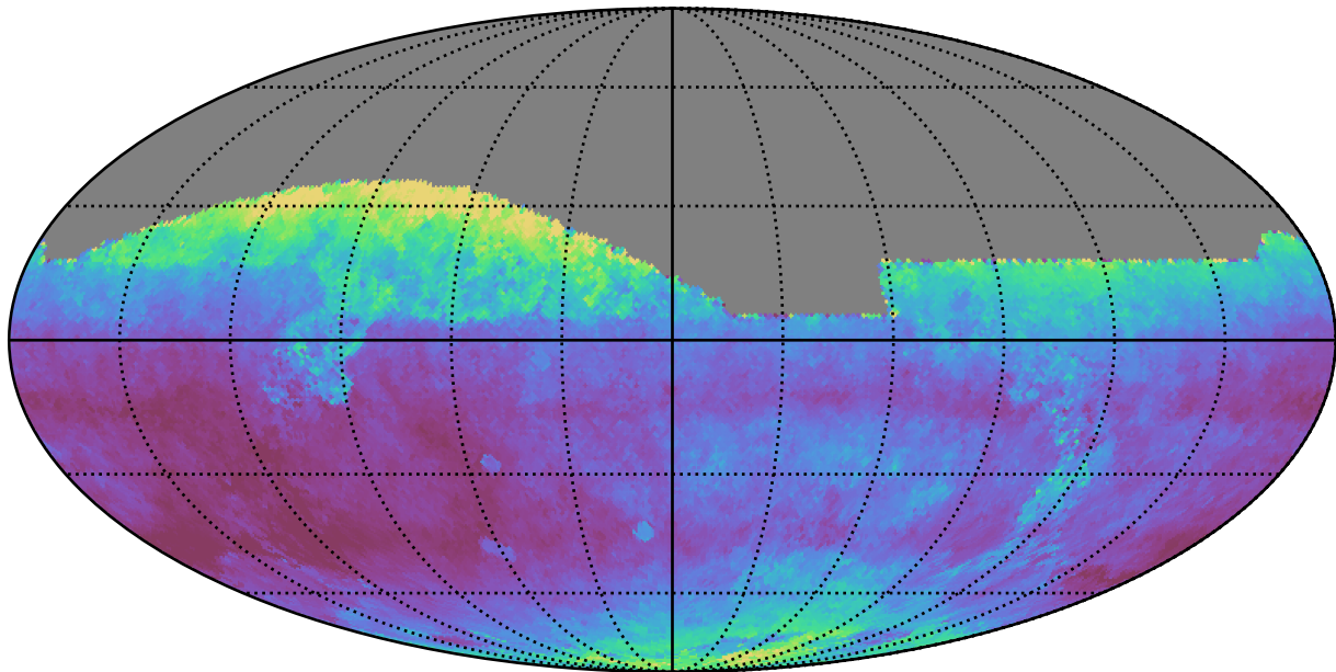
weather_cloudso4v3.4_10yrs All sky i band: Median seeingEff
