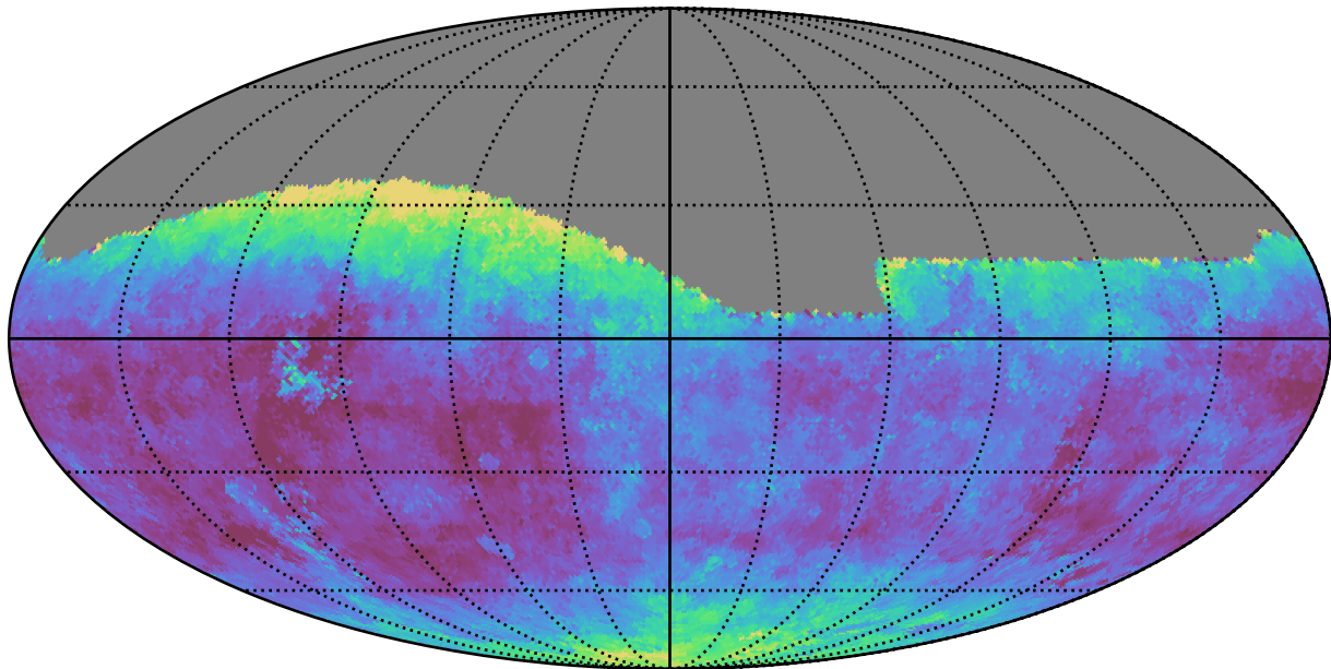
weather_cloudso4v3.4_10yrs All sky g band: Median seeingEff
