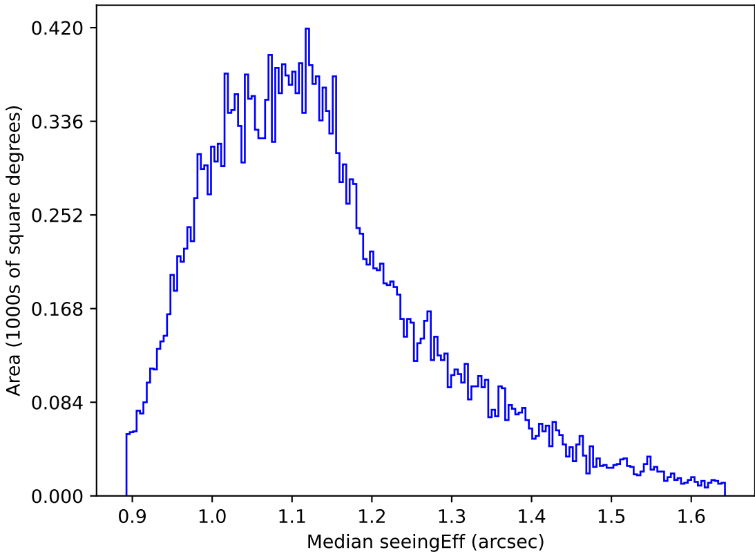
weather_cloudso4v3.4_10yrs All sky g band: Median seeingEff
