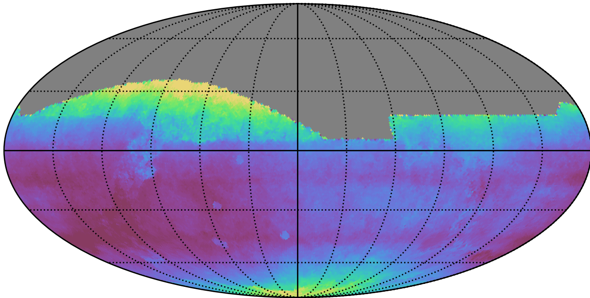
weather_cloudso4v3.4_10yrs All sky all bands: Median seeingEff
