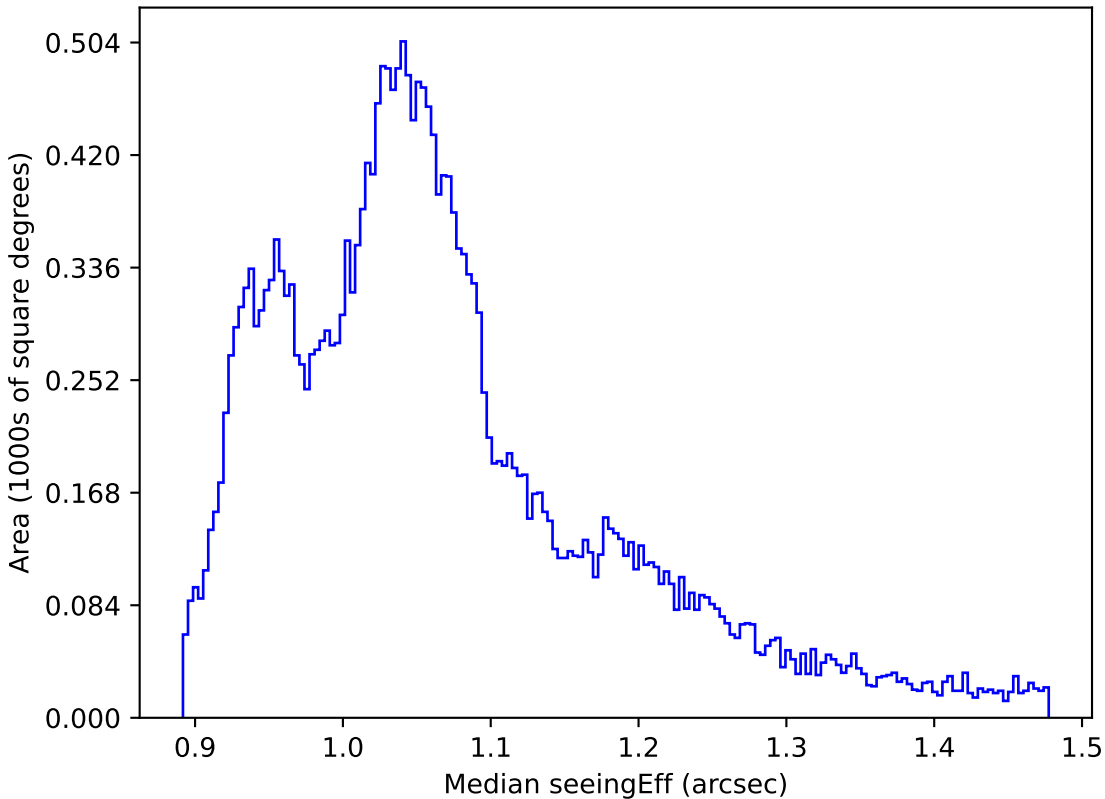
weather_cloudso4v3.4_10yrs All sky all bands: Median seeingEff
