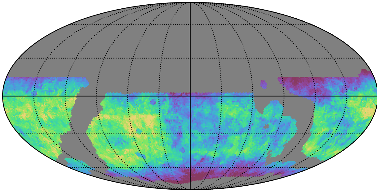
weather_cloudso4v3.4_10yrs WFD g band: Median saturation_mag
