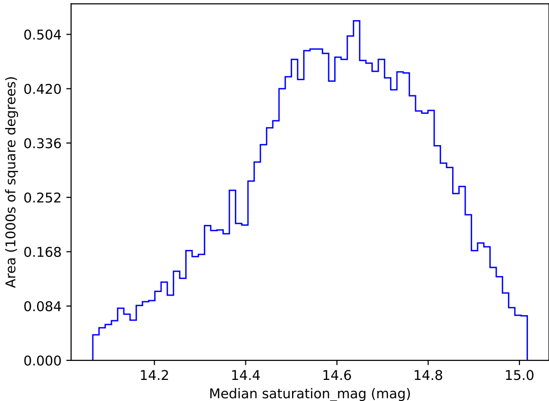
weather_cloudso4v3.4_10yrs WFD g band: Median saturation_mag
