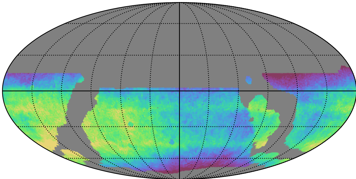
weather_cloudso4v3.4_10yrs WFD all bands: Median saturation_mag
