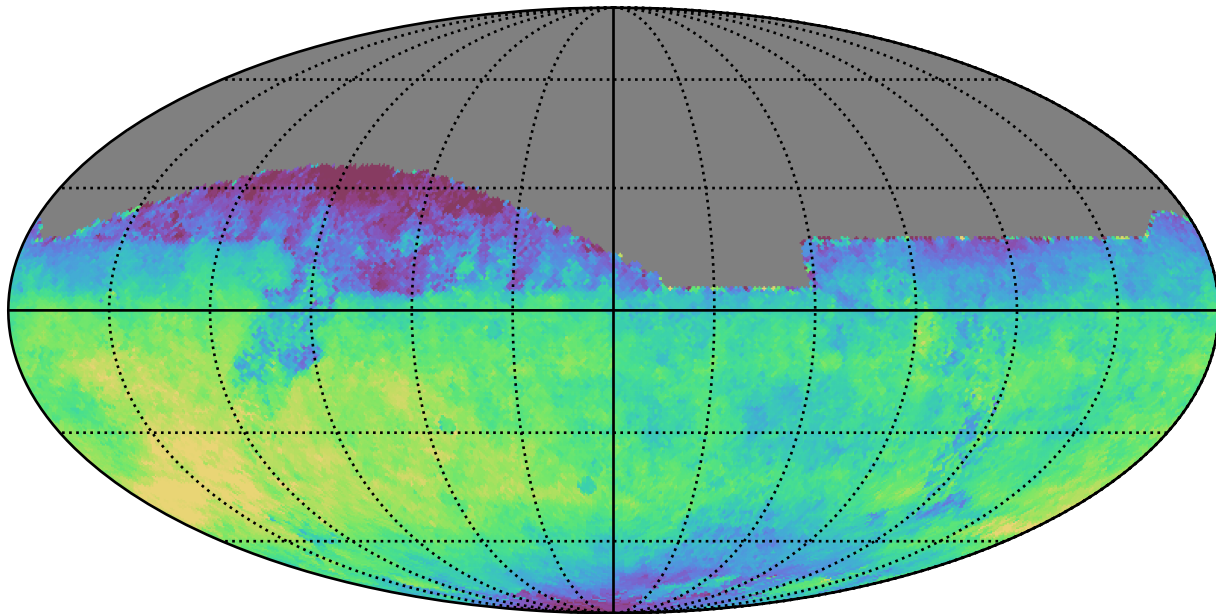
weather_cloudso4v3.4_10yrs All sky z band: Median saturation_mag
