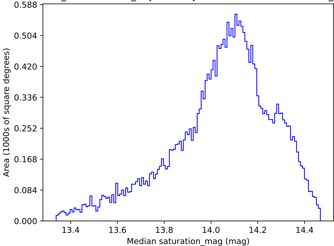
weather_cloudso4v3.4_10yrs All sky z band: Median saturation_mag
