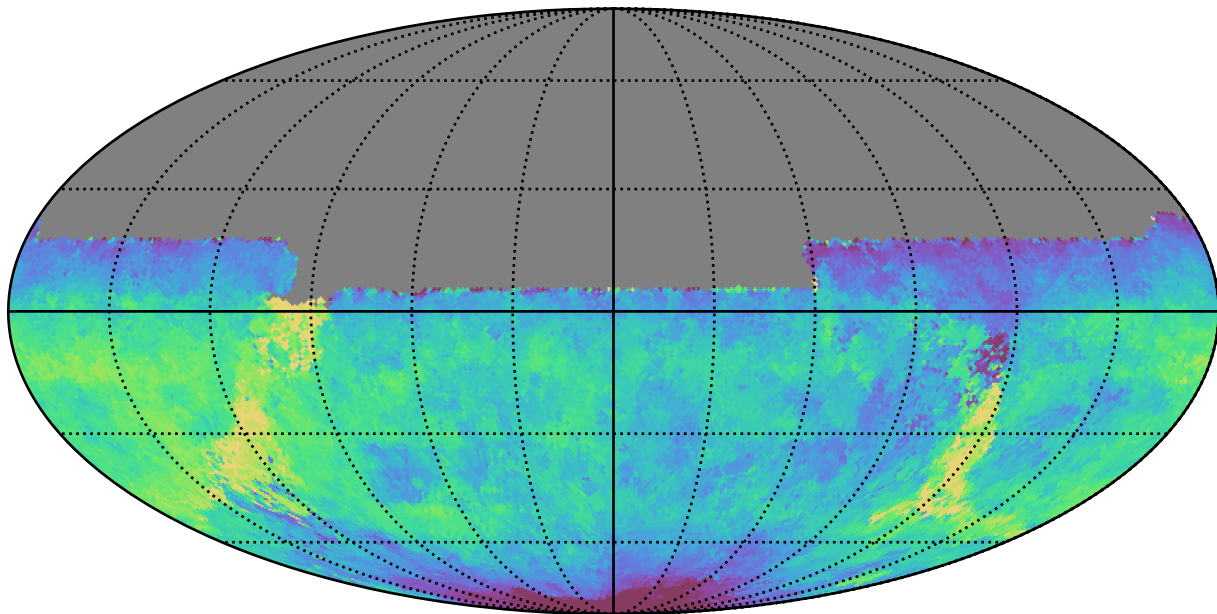
weather_cloudso4v3.4_10yrs All sky u band: Median saturation_mag
