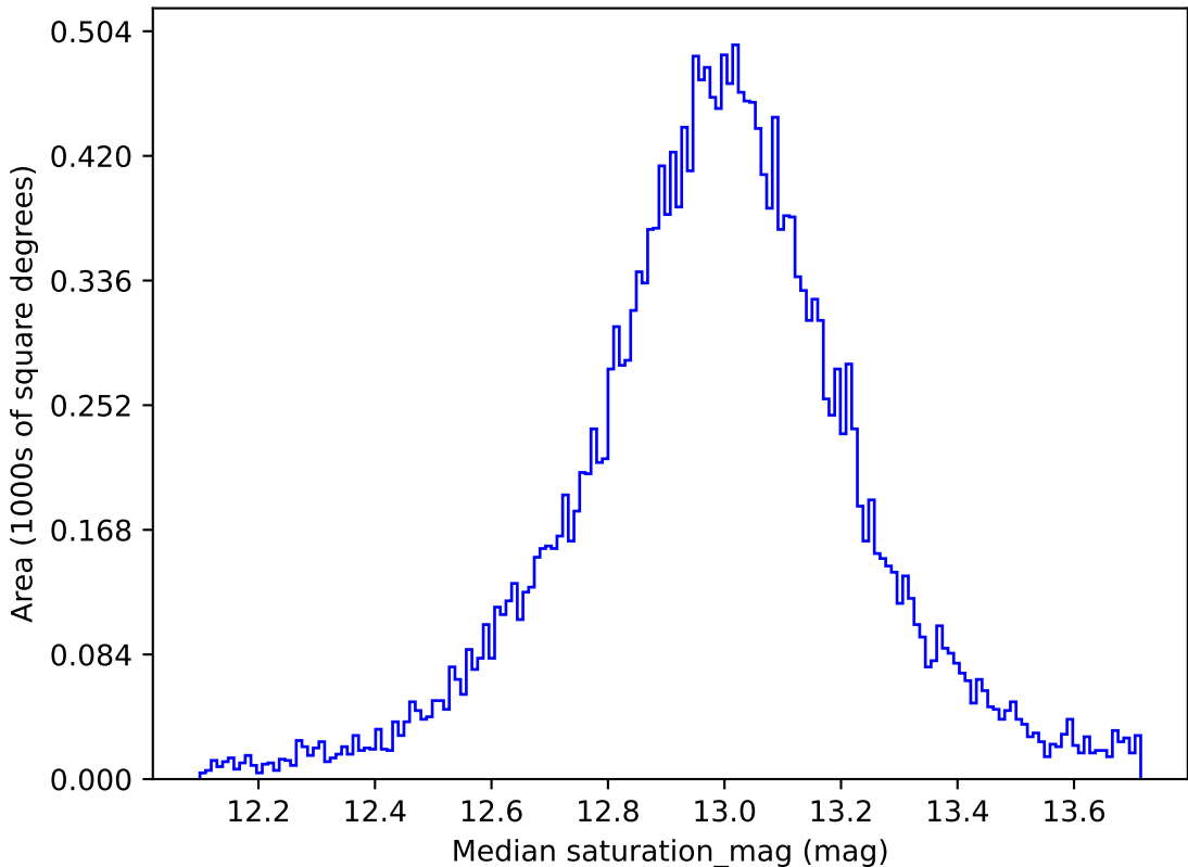
weather_cloudso4v3.4_10yrs All sky u band: Median saturation_mag
