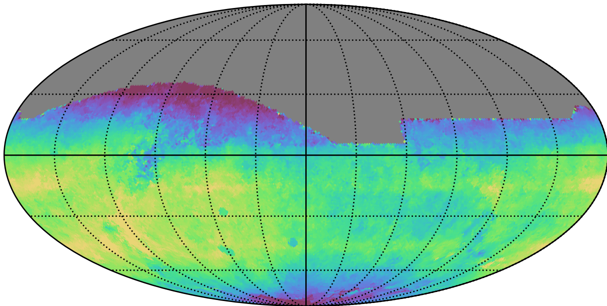
weather_cloudso4v3.4_10yrs All sky r band: Median saturation_mag
