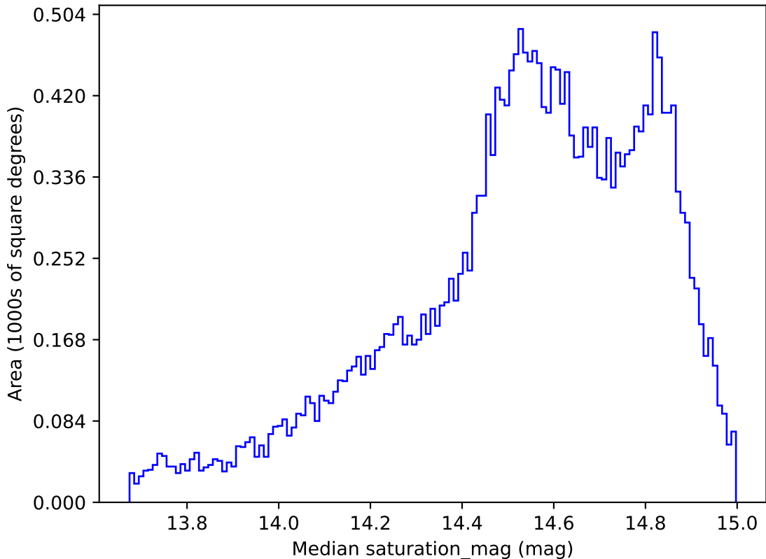
weather_cloudso4v3.4_10yrs All sky r band: Median saturation_mag
