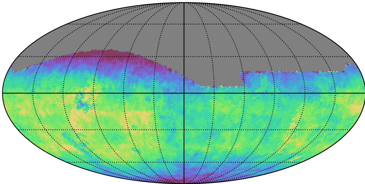
weather_cloudso4v3.4_10yrs All sky g band: Median saturation_mag
