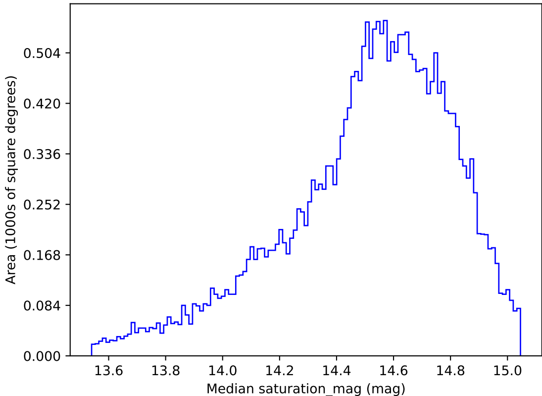
weather_cloudso4v3.4_10yrs All sky g band: Median saturation_mag
