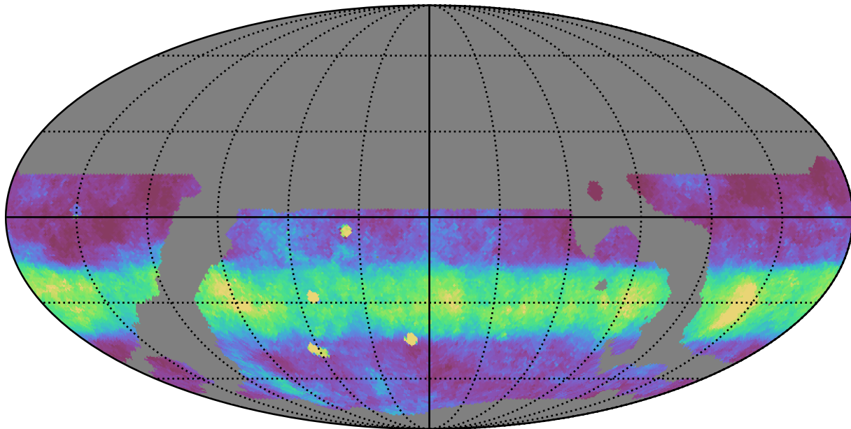
weather_cloudso4v3.4_10yrs WFD z band: Median normairmass
