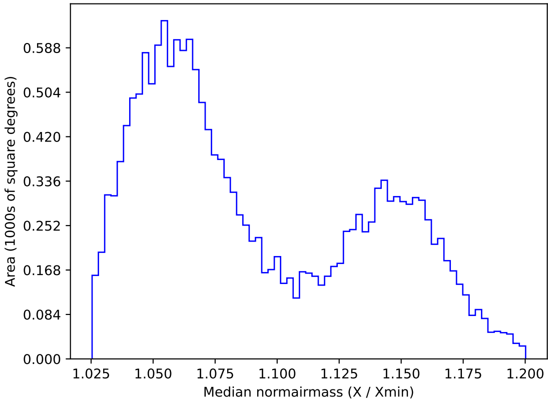
weather_cloudso4v3.4_10yrs WFD z band: Median normairmass
