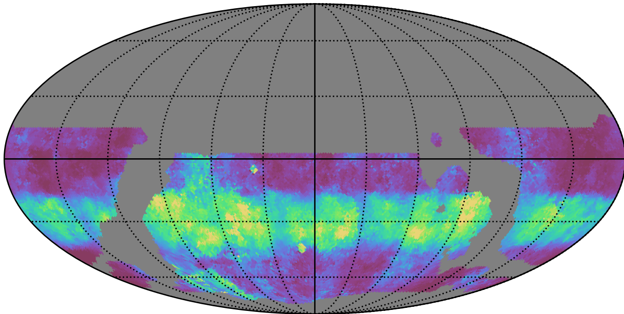
weather_cloudso4v3.4_10yrs WFD u band: Median normairmass
