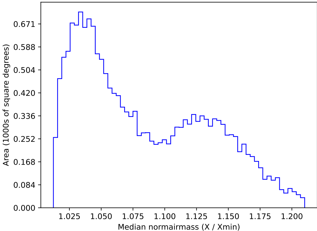
weather_cloudso4v3.4_10yrs WFD u band: Median normairmass
