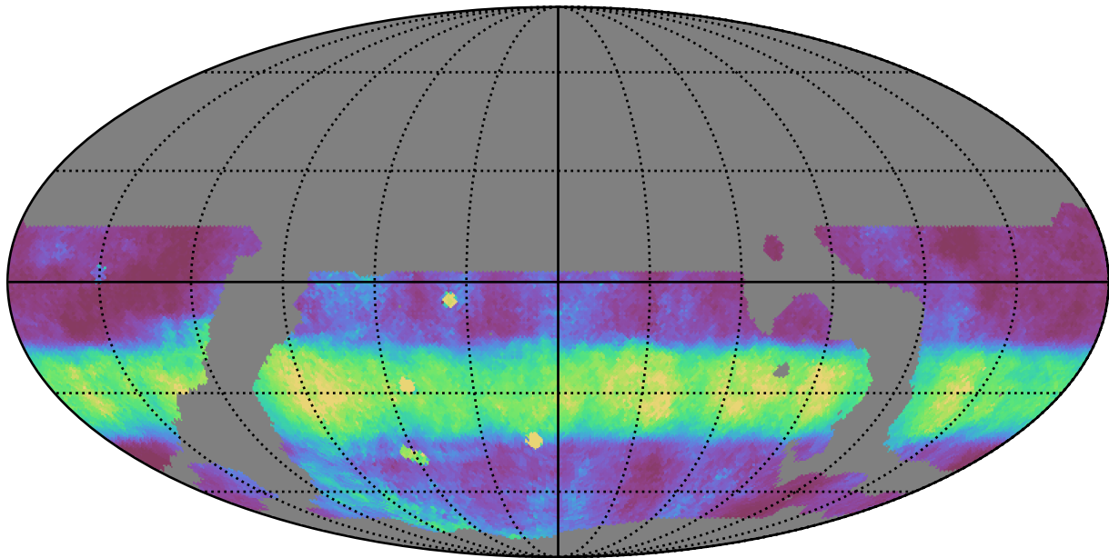
weather_cloudso4v3.4_10yrs WFD r band: Median normairmass
