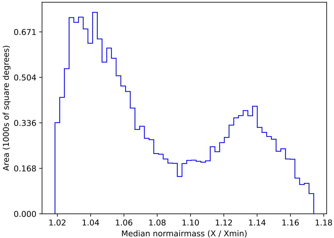
weather_cloudso4v3.4_10yrs WFD r band: Median normairmass
