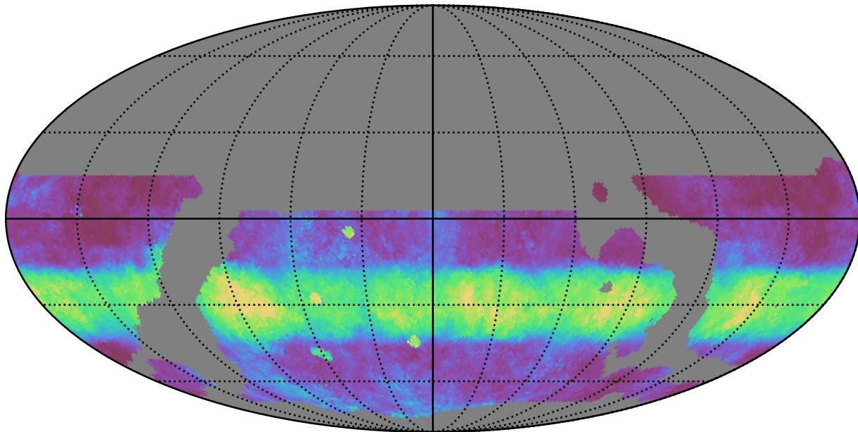
weather_cloudso4v3.4_10yrs WFD i band: Median normairmass
