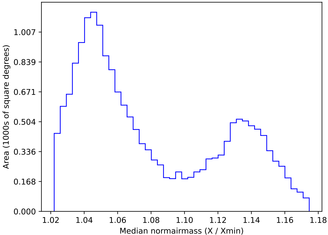
weather_cloudso4v3.4_10yrs WFD i band: Median normairmass
