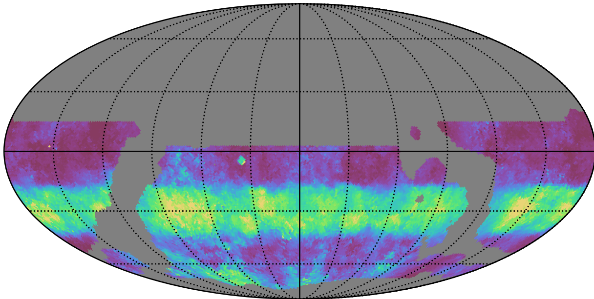
weather_cloudso4v3.4_10yrs WFD g band: Median normairmass
