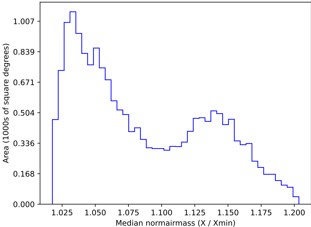
weather_cloudso4v3.4_10yrs WFD g band: Median normairmass
