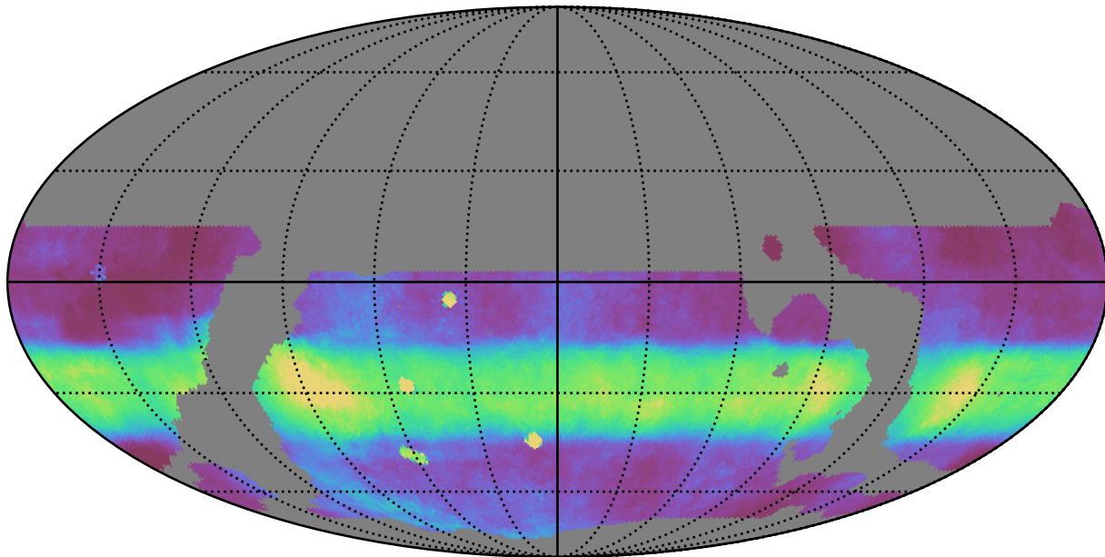
weather_cloudso4v3.4_10yrs WFD all bands: Median normairmass
