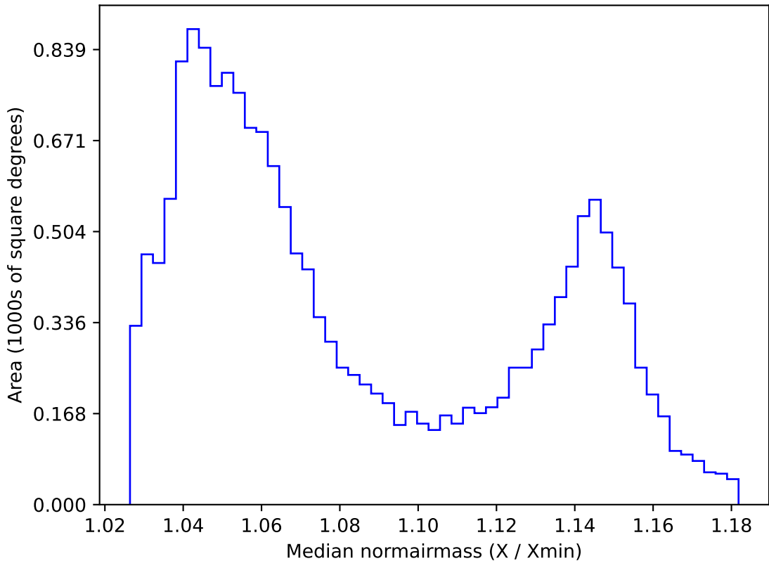
weather_cloudso4v3.4_10yrs WFD all bands: Median normairmass
