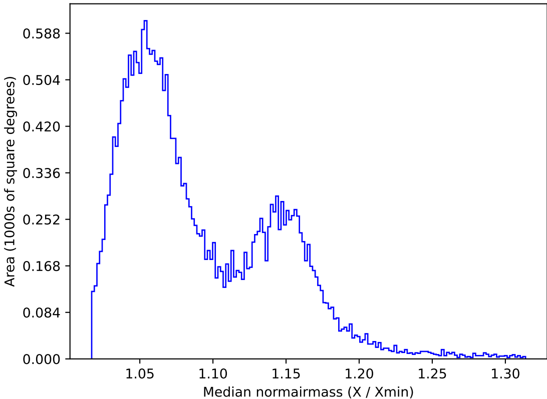
weather_cloudso4v3.4_10yrs All sky z band: Median normairmass
