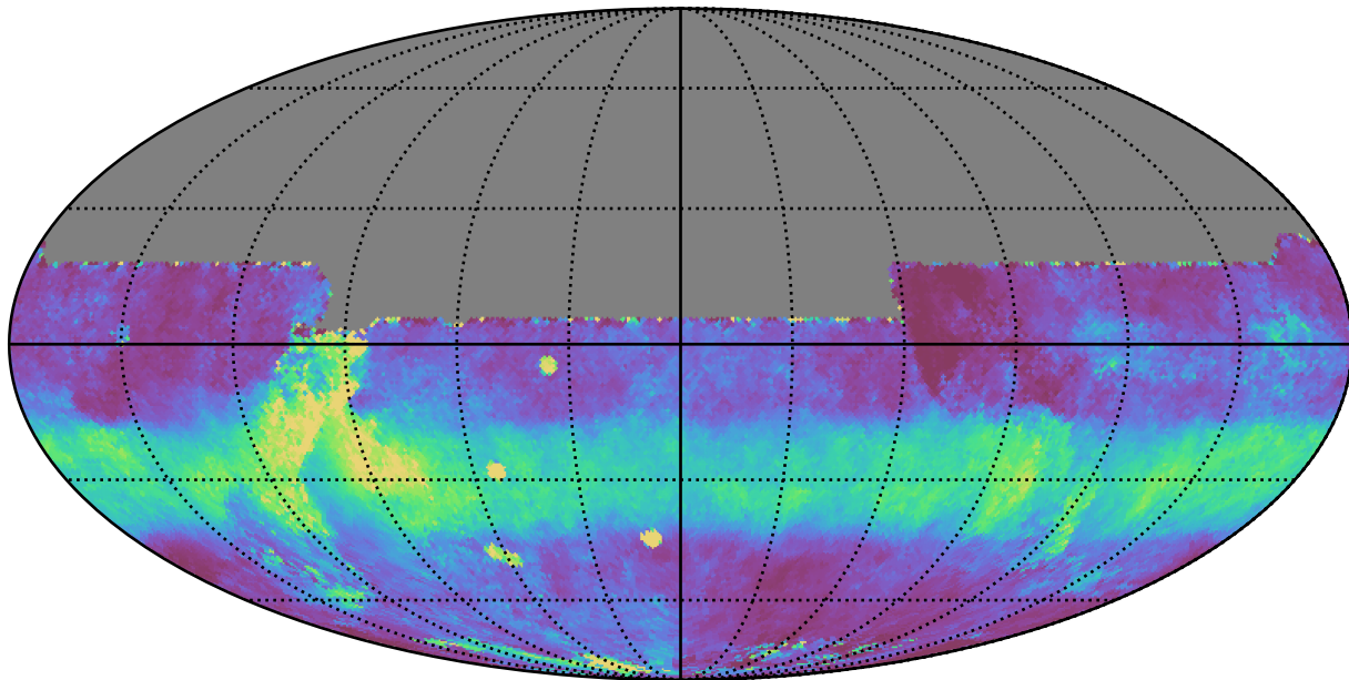
weather_cloudso4v3.4_10yrs All sky y band: Median normairmass
