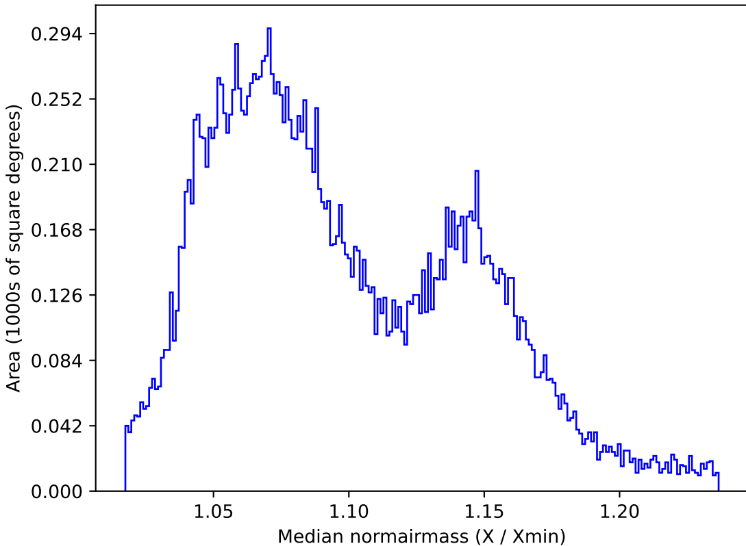
weather_cloudso4v3.4_10yrs All sky y band: Median normairmass
