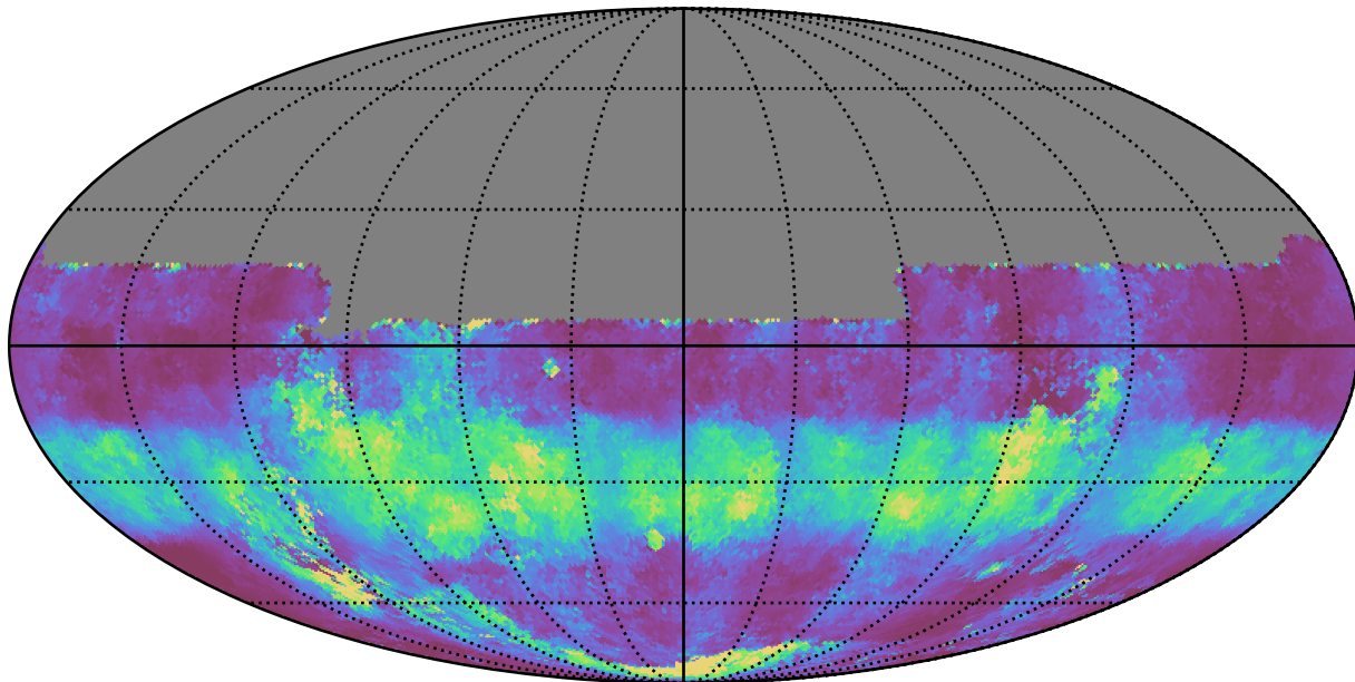
weather_cloudso4v3.4_10yrs All sky u band: Median normairmass
