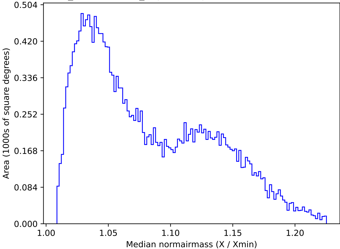
weather_cloudso4v3.4_10yrs All sky u band: Median normairmass
