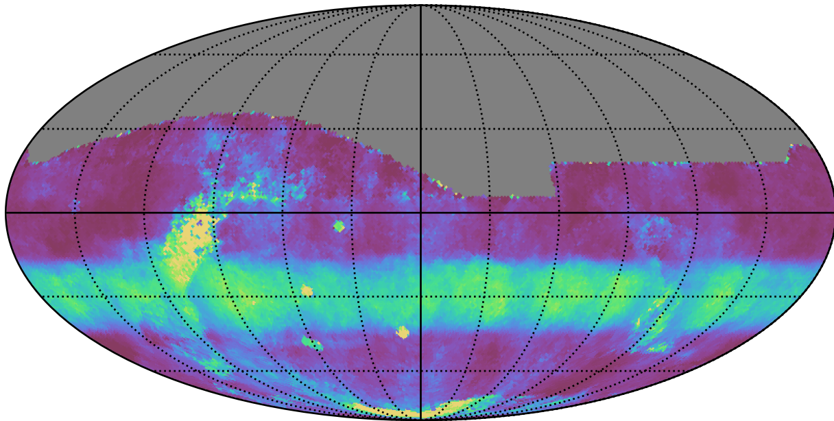
weather_cloudso4v3.4_10yrs All sky r band: Median normairmass
