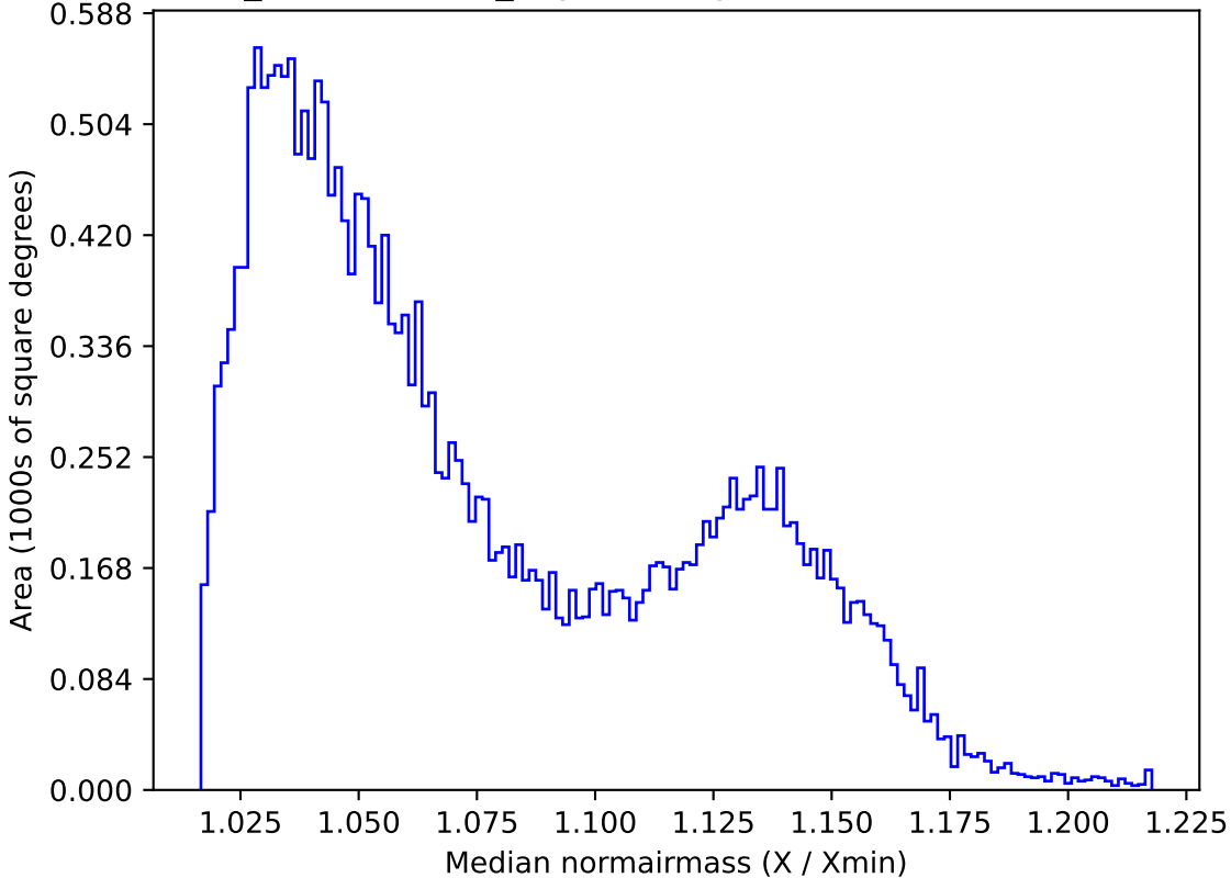
weather_cloudso4v3.4_10yrs All sky r band: Median normairmass
