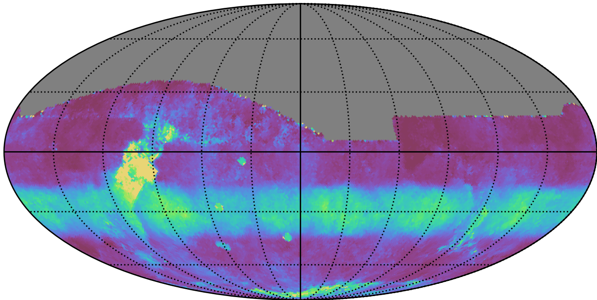
weather_cloudso4v3.4_10yrs All sky i band: Median normairmass
