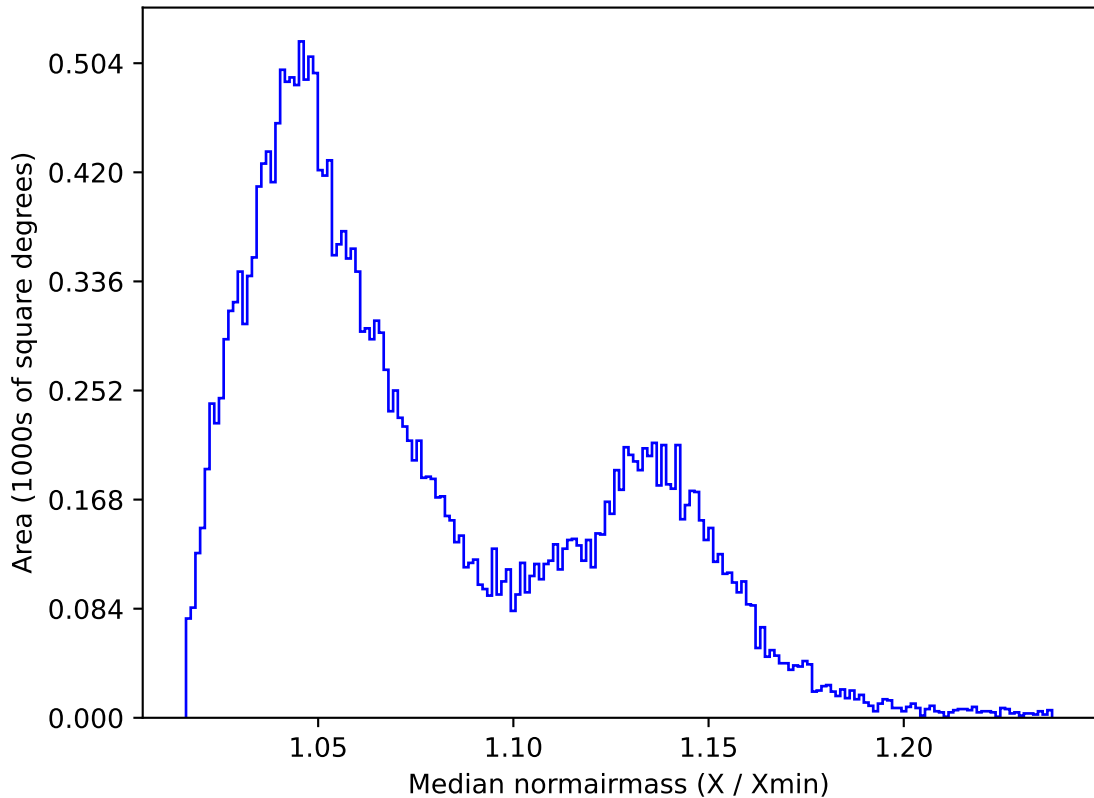
weather_cloudso4v3.4_10yrs All sky i band: Median normairmass
