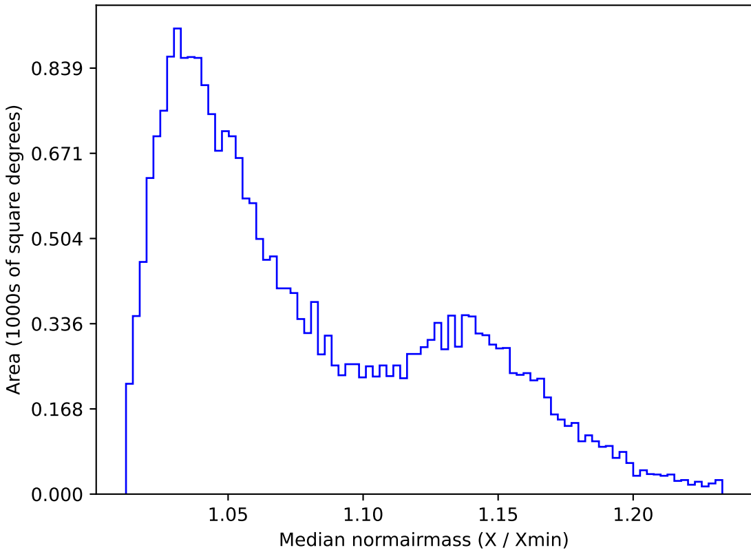
weather_cloudso4v3.4_10yrs All sky g band: Median normairmass
