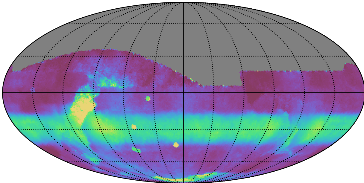
weather_cloudso4v3.4_10yrs All sky all bands: Median normairmass
