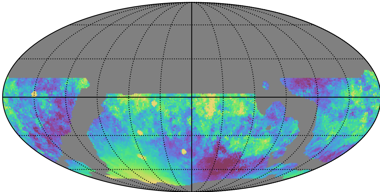
weather_cloudso4v3.4_10yrs WFD z band: Median moonDistance
