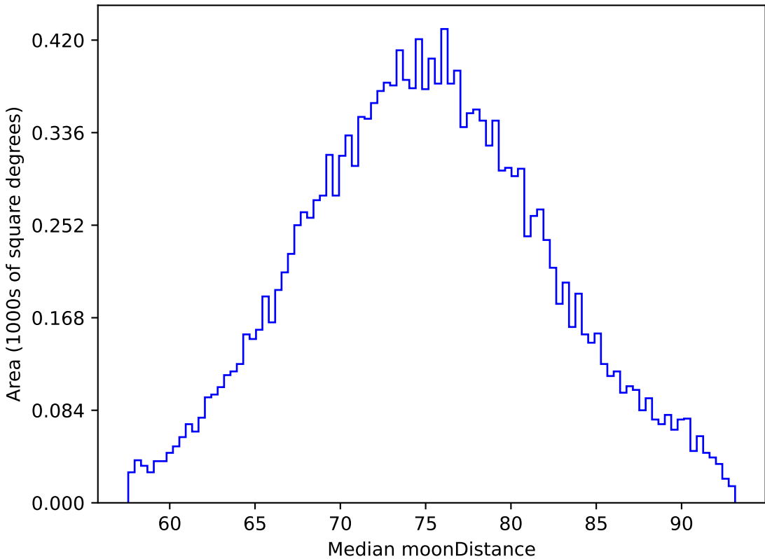
weather_cloudso4v3.4_10yrs WFD z band: Median moonDistance
