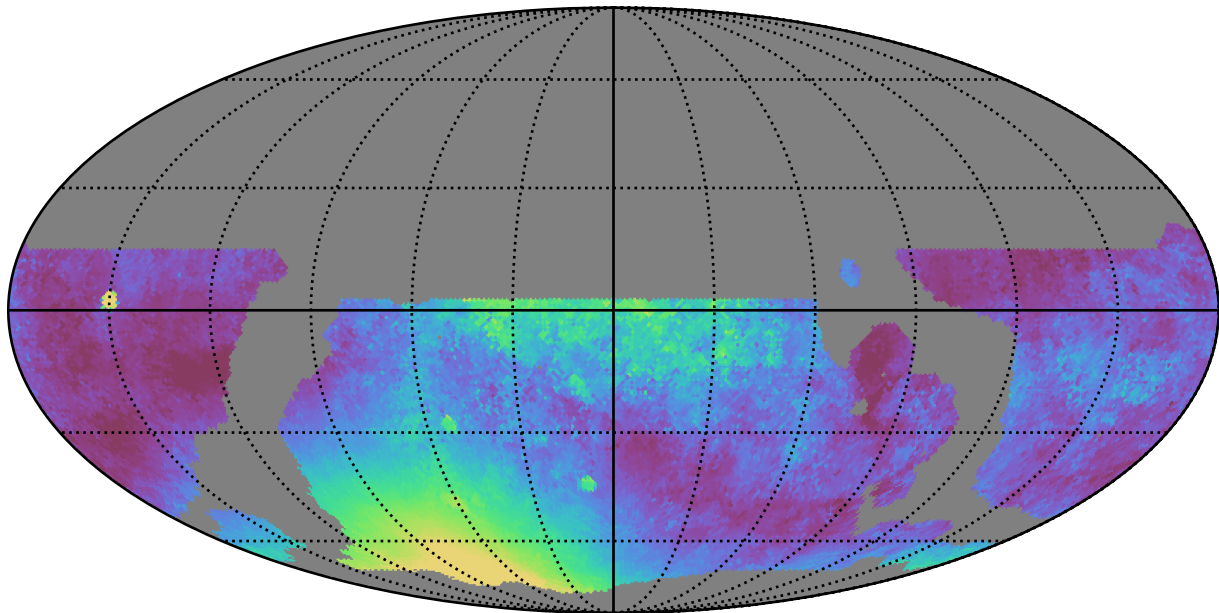
weather_cloudso4v3.4_10yrs WFD y band: Median moonDistance
